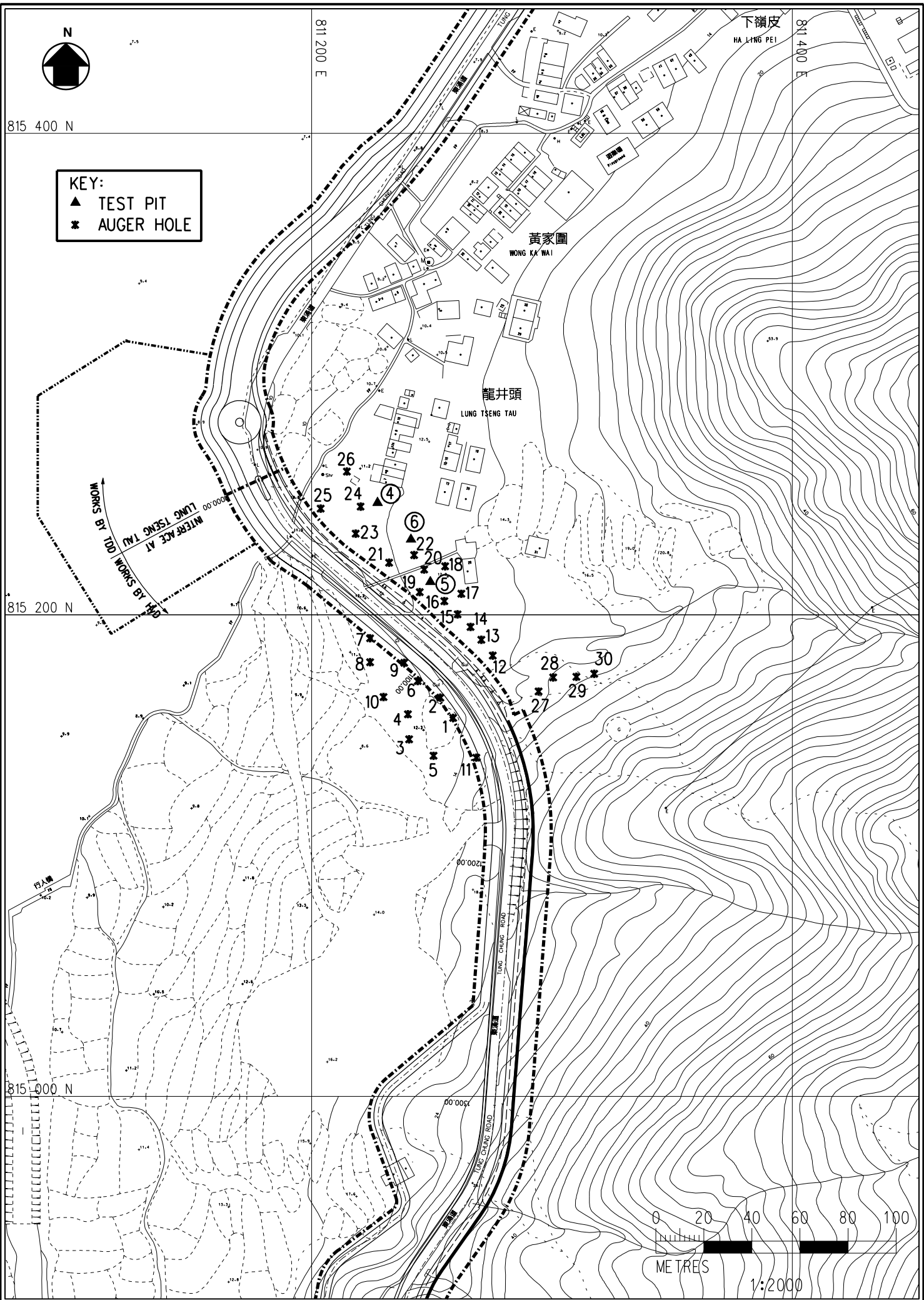
LOCATION OF AUGER TESTS AND TEST PITS 4, 5 AND 6 IN TUNG CHUNG (AREA 1)
